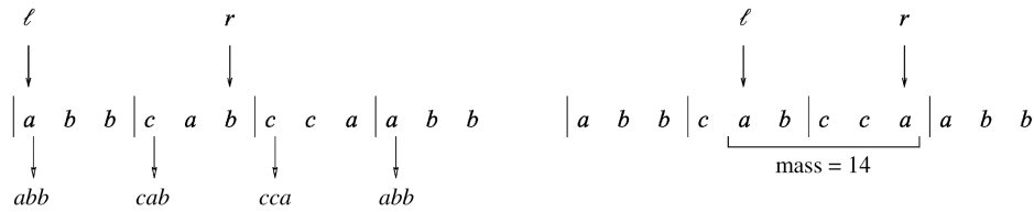
Fig. 1. Example 1—LOOKUP searching for M = 14 .
